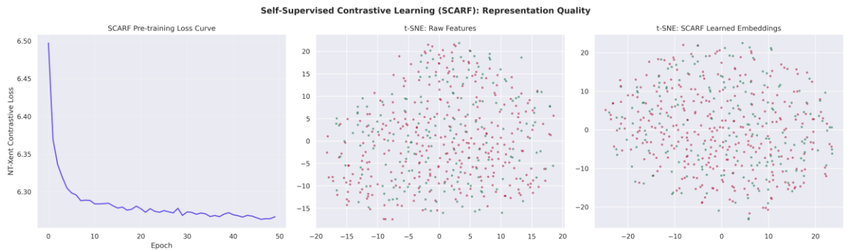
Figure 40: SCARF Self-Supervised Latent Embeddings t-SNE Dimensionality Projections
